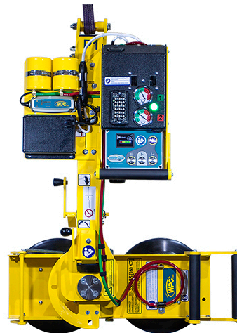
90° locked rotation
